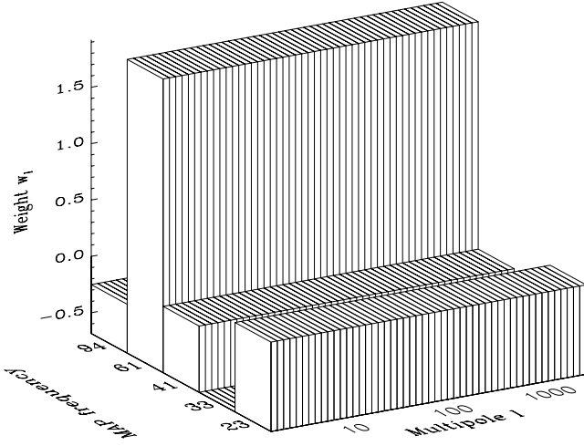
FIG. 3. The weights w_\ell used to create the internal linear combination map of the WMAP team are independent of angular scale. The figure shows the weights w_\ell = (0.109, -0.684, -0.096, 1.921, -0.250) used outside of the galactic plane.
